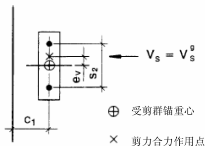
图4.4.2-5 偏心受剪举例[4]
